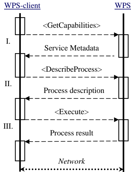
Figure 1: Basic client-service communication in WPS.
